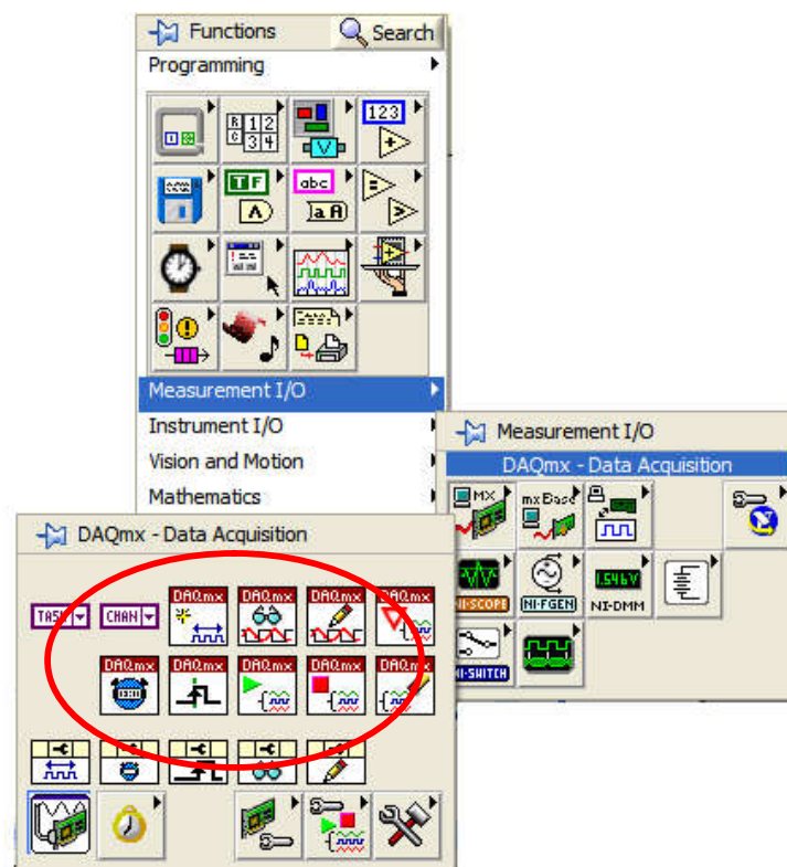
Sl. 4.2.5. DAQmx Vis: Functions»Measurement I/O»DAQmx – Data Acquisition
